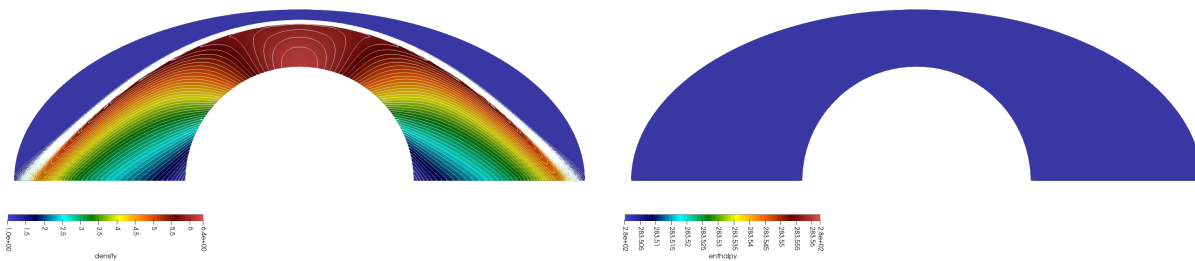
FIGURE 1: Density (left) and total enthalpy (right) for the mach 20 flow around a cylinder. The density field matches the reference solutions of the literature, while the enthalpy field is constant in the whole domain. The correction proposed here preserves enthalpy.
