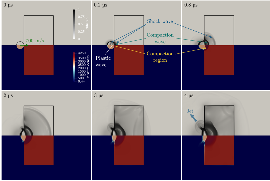
FIGURE 1: Two-dimensional impact of an aluminum cylinder (diameter 2 mm, velocity 700 \text{ ms}^{-1} ) on a porous titanium plate (20% initial porosity). The titanium target has dimensions 8 \text{ mm} \times 16 \text{ mm} and is embedded in a 24 \text{ mm} \times 24 \text{ mm} computational domain with non-reflecting boundary conditions. Initial pressure is 10^5 \text{ Pa} and densities are \rho_{\text{air}} = 1.2 \text{ kg m}^{-3} , \rho_{\text{alu}} = 2700 \text{ kg m}^{-3} and \rho_{\text{tit}} = 4527 \text{ kg m}^{-3} . Both materials follow a GTN plasticity model. The simulation is performed on a 400 \times 400 Cartesian grid using a second-order finite-volume scheme with van Leer limiter [2]. Top: numerical Schlieren visualisation highlighting wave structures. Bottom: mixture density showing compaction. Snapshots are shown at t = 0.2, 0.8, 2, 3 and 4 \mu\text{s} . After impact, strong shock and compaction waves propagate in both materials. While compaction in aluminum remains limited, the porous titanium undergoes rapid pore collapse, leading to a nearly fully compacted state. Wave attenuation is observed in the aluminum due to multiple reflections, whereas the compaction front in titanium remains well defined and propagates through the plate. At later times, the shock reaches the rear surface, generating transmitted and reflected waves and complex interactions inside the target. The aluminum cylinder experiences severe plastic deformation and flattening, accompanied by lateral jetting and a leading shock in the surrounding air. This test case illustrates the ability of the model to capture large deformations, shock interactions and irreversible compaction of porous materials within a unified framework.
